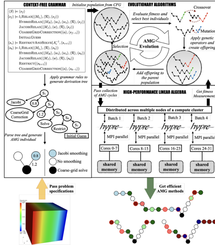
Figure 1 (reproduced from [1]): Automatic design of algebraic multigrid (AMG) solvers using grammar-guided evolution. Given an input problem, the approach combines a context-free grammar, an evolutionary algorithm and high-performance solvers to generate flexible AMG cycles. Nodes in the resulting cycles are colour-coded by smoothing operation. In this project, neural networks will learn from previous searches to guide this process.
